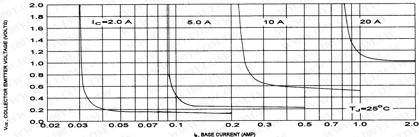
"ON" VOLTAGES
