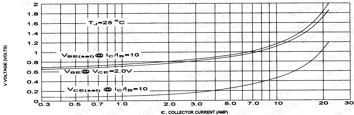
"ON" VOLTAGES
