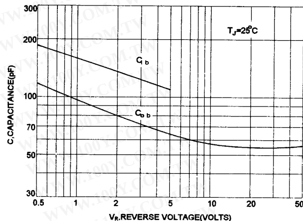
FIG-8 CAPACITANCES
