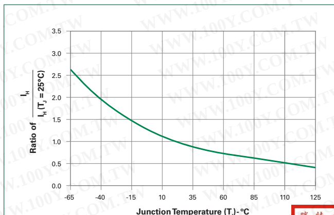
Figure 3: Normalized DC Holding Current vs. Junction Temperature
