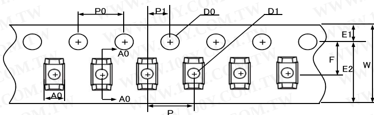
Component Orientation in Tape
