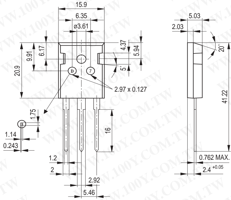
P-TO-247-3-1
