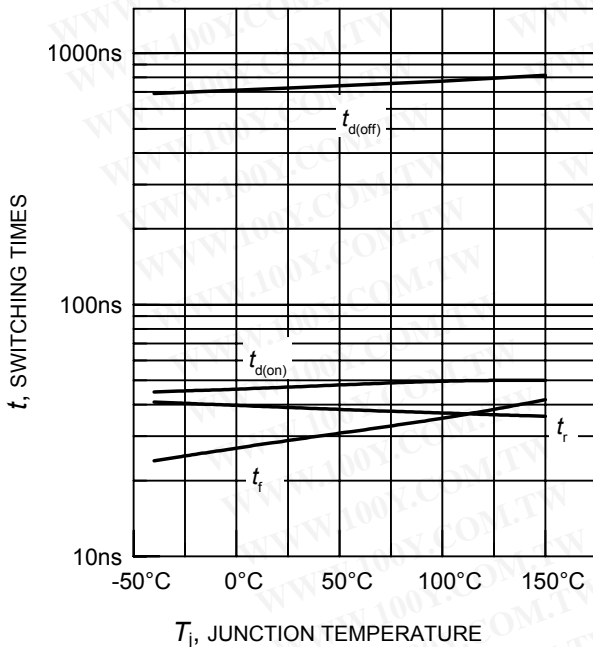
Figure 11. Typical switching times as a function of junction temperature (inductive load, V_{CE} = 800\text{V} , V_{GE} = +15\text{V}/0\text{V} , I_C = 25\text{A} , R_G = 22\ \Omega , dynamic test circuit in Fig.E )
