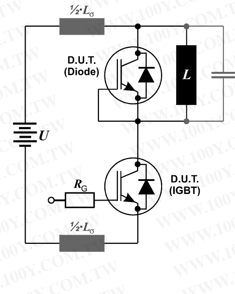
Figure E. Dynamic test circuit Leakage inductance L_{\sigma}=180\text{nH} , and stray capacity C_{\sigma}=40\text{pF} .
