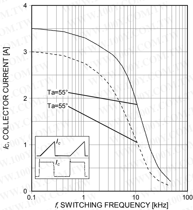
Figure 1. Collector current as a function of switching frequency ( T_{vj} \leq 175^\circ\text{C} , D=0.5 , V_{CE}=400\text{V} , V_{GE}=15/0\text{V} , r_G=43\Omega , PCB Mounting, 6\text{cm}^2 Cu, P_{tot}=2,4\text{W} )
