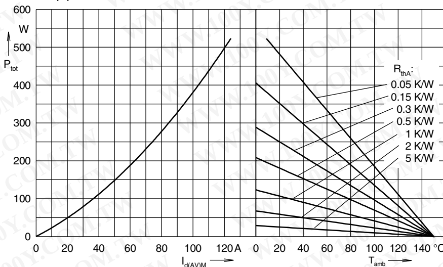
Fig. 4 Power dissipation versus direct output current and ambient temperature, \sin \phi = 1
