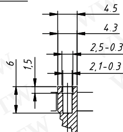
Detail Z
