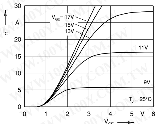
Fig. 7 Typ. output characteristics
