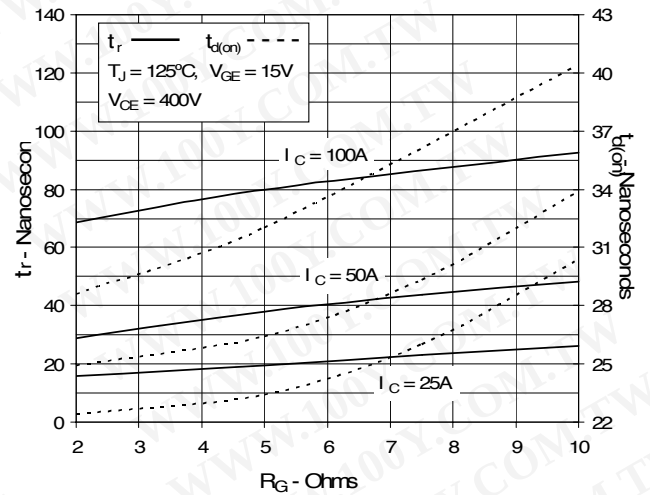
Fig. 14. Inductive Turn-on Switching Times vs. Gate Resistance
