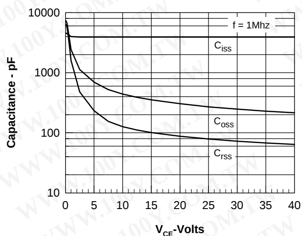
Figure 6. Capacitance Curves
