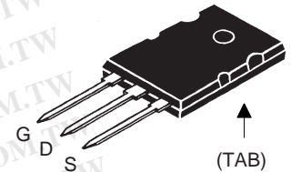
TO-264 (IXFK)
