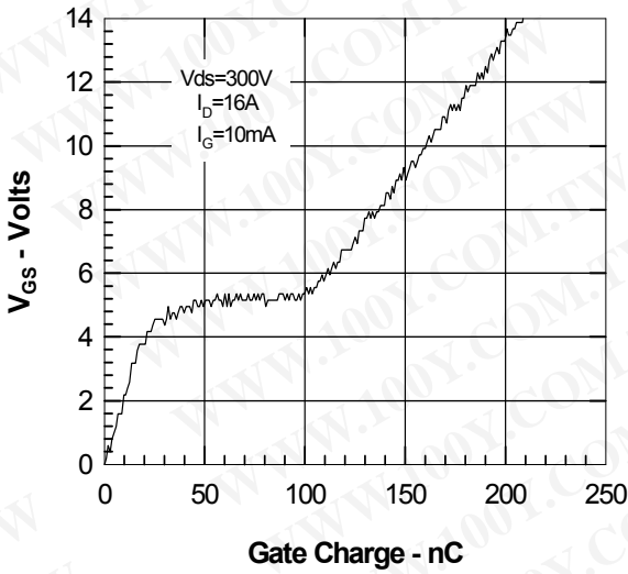
Figure 7. Gate Charge
