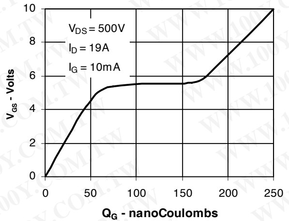
Fig. 10. Gate Charge
