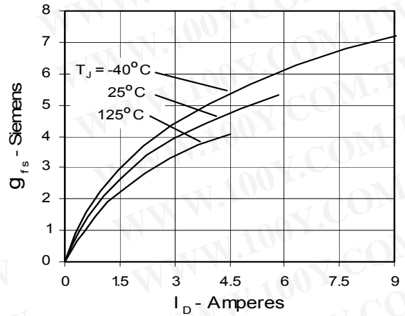
Fig. 8. Transconductance
