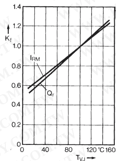
Fig. 4 Dynamic parameters versus junction temperature.
