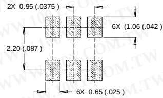
RECOMMENDED FOOTPRINT
