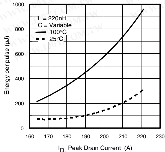
Fig 6. Typical E_{PULSE} vs. Peak Drain Current
