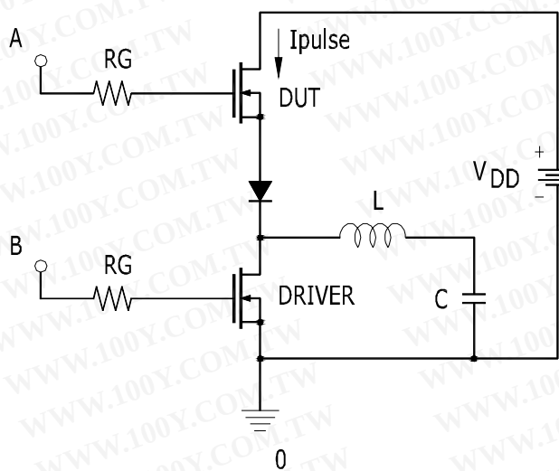
Fig 21a. t_{st} and E_{PULSE} Test Circuit
