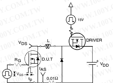
Fig 19a. Unclamped Inductive Test Circuit
