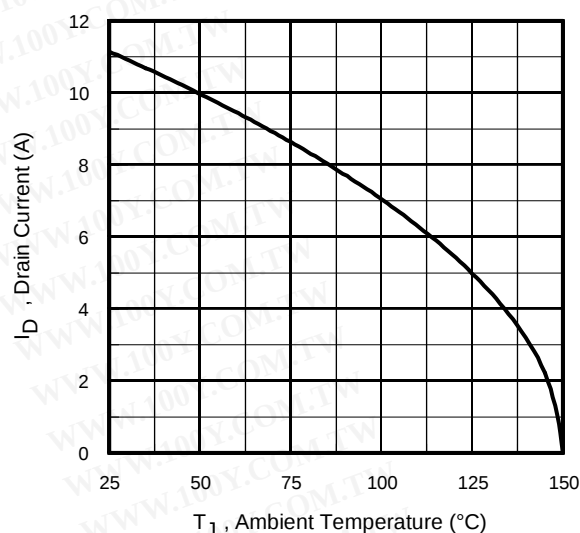
Fig 20. Maximum Drain Current vs. Ambient Temp.
