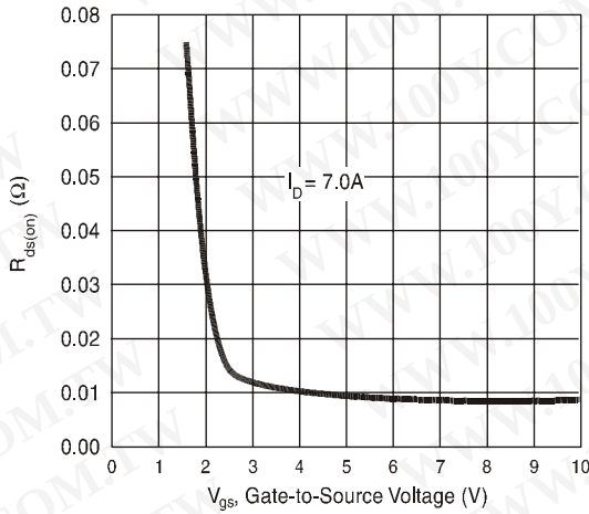
Fig 3. Typical R_{DS(on)} vs. Gate-to-Source Voltage
