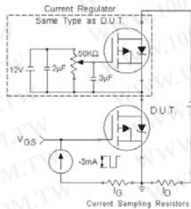
Fig 9b. Gate Charge Test Circuit
