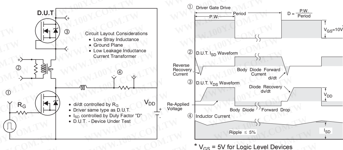
Fig 17. Diode Reverse Recovery Test Circuit for N-Channel HEXFET® Power MOSFETs
