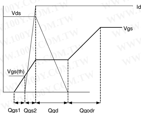
Fig 16b. Gate Charge Waveform
