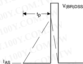
Fig 18b. Unclamped Inductive Waveforms
