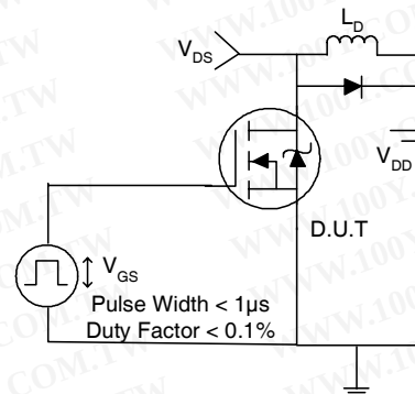
Fig 14a. Switching Time Test Circuit
