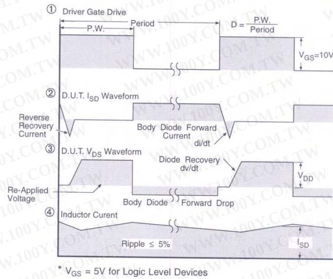
Fig 14. For N-Channel HEXFETS
