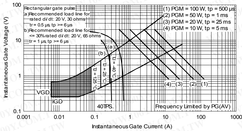
Fig. 8 - Gate Characteristics
