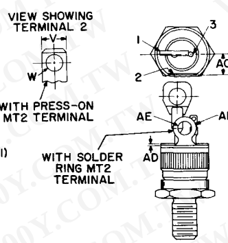
ISOLATED STUD TYPE 3
