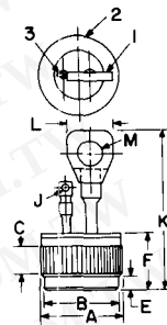
FIGURE B (Flag MT1 Terminal)
