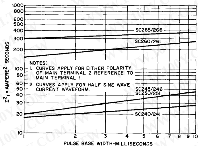
9. I^2t RATING FOLLOWING RATED LOAD CONDITIONS
