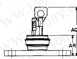
NON-ISOLATED TO-3 FLANGE TYPE 5
