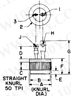
FIGURE A (Pierced MT1 Terminal)
