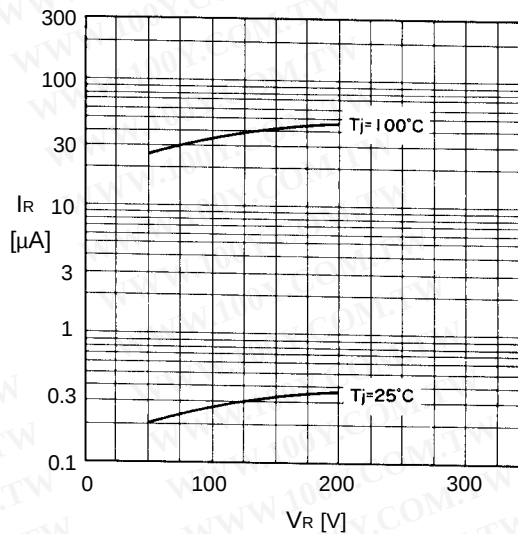
Reverse characteristics
