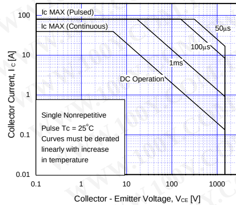
Fig 14. SOA Characteristics
