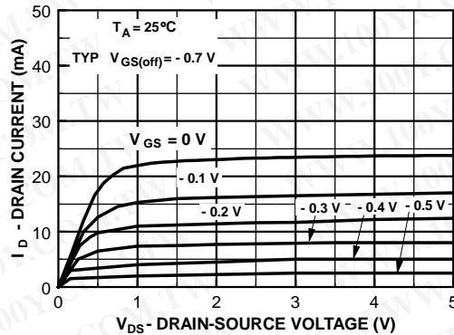
Figure 4. Common Drain-Source
