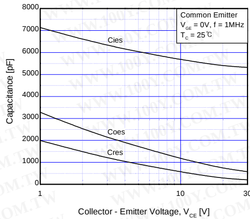
Fig 7. Capacitance Characteristics
