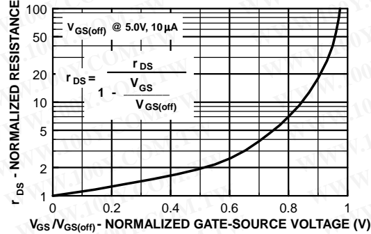
Normalized Drain Resistance vs Bias Voltage
