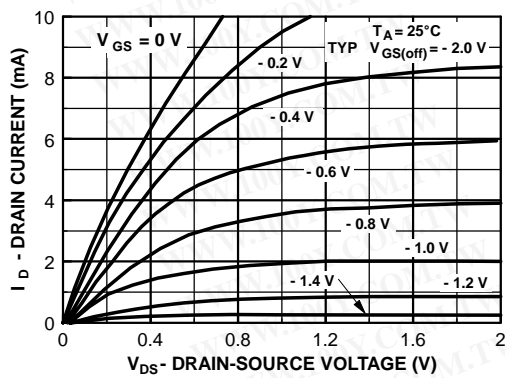
Common Drain-Source
