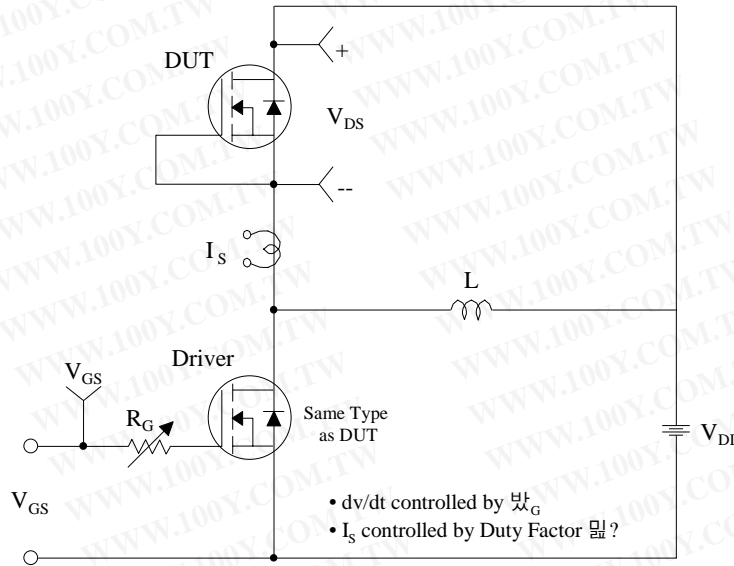
Fig 15. Peak Diode Recovery dv/dt Test Circuit & Waveforms
