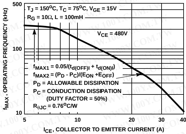
FIGURE 13. OPERATING FREQUENCY vs COLLECTOR TO EMITTER CURRENT T
