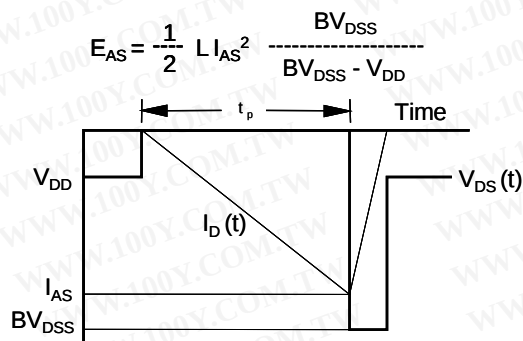
Unclamped Inductive Switching Test Circuit &amp; Waveforms
