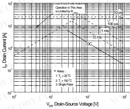
Figure 9-1. Maximum Safe Operating Area for FQP6N90C
