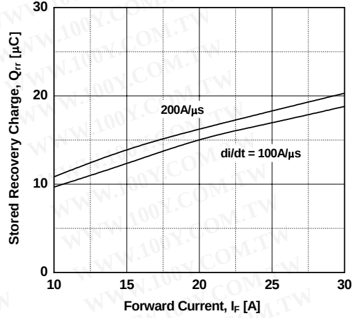
Figure 20. Stored Charge
