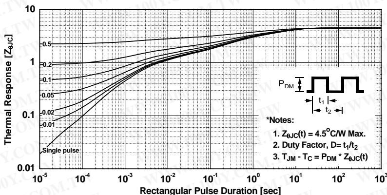
Figure 13. Transient Thermal Response Curve - FDPF5N50
