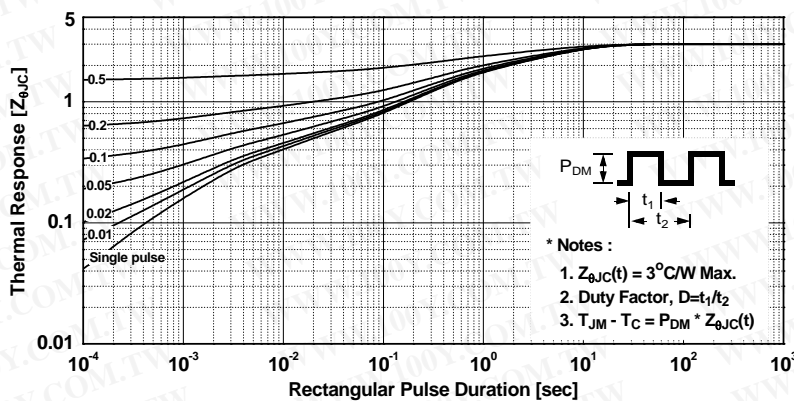
Figure 11-2. Transient Thermal Response Curve - FDPF12N50
