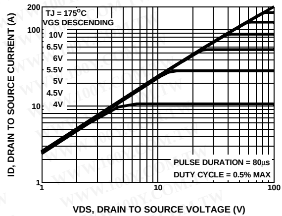
Figure 2. Output Characteristics
