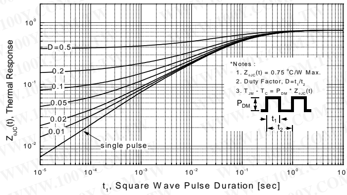
Figure 11-1. Transient Thermal Response Curve (FCP16N60)
