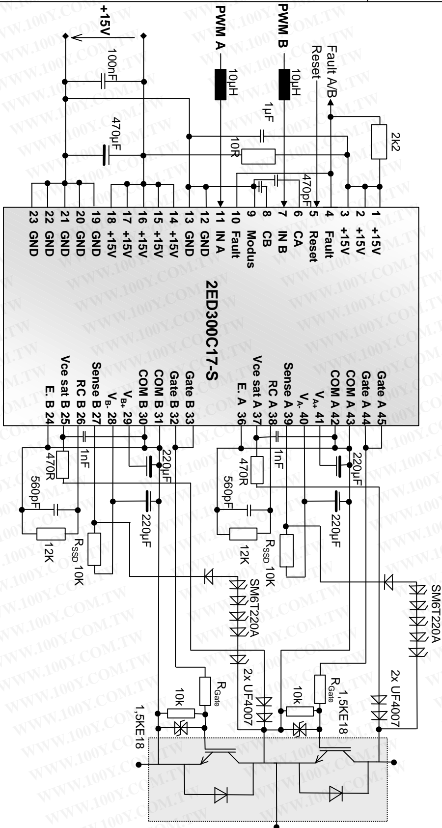
Fig. 3.12 Commissioning circuit in the direct mode: (Both channels can be switched independently)
