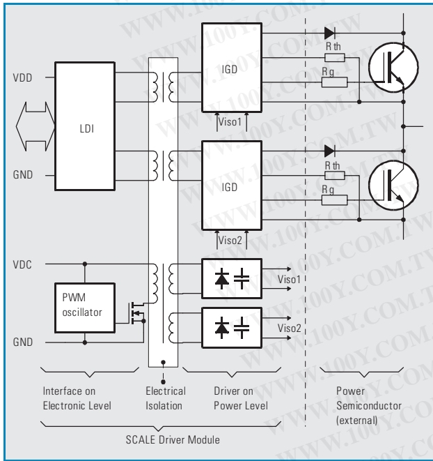
Block diagram shows 2 channels (i.e. one third of the 6SD 106E1-17)
