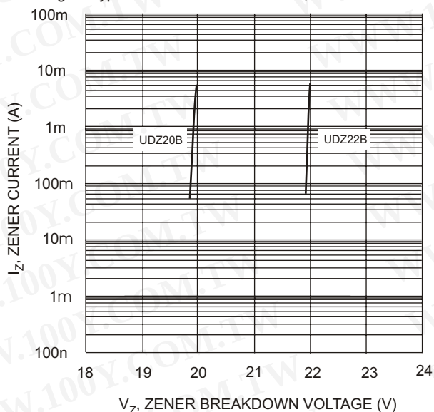
Fig. 5 Typical Reverse Characteristics, UDZ20B - UDZ22B
