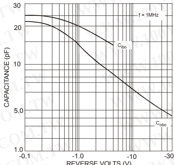
Fig. 6 Typical Capacitance
