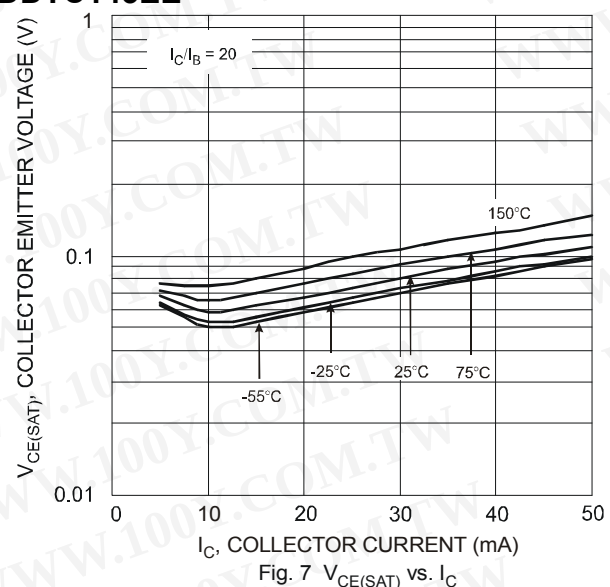
Fig. 7 V_{CE(SAT)} vs. I_C
